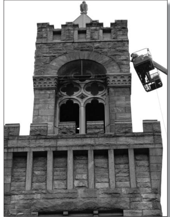
Condition assessment and nondestructive testing of a stone facade
