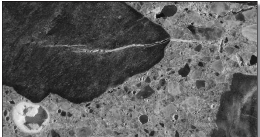
Microscopic concrete petrographic examination
